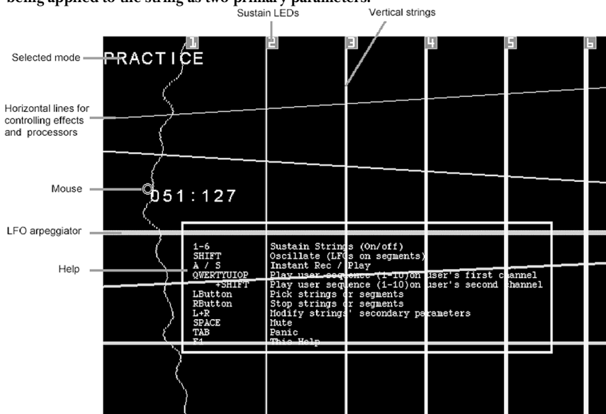
Fig. 2a. Bamboo snapshot: plucking the leftmost string with the mouse while pressing HELP (F1). The circle shows the mouse position and, next to it, its instant values that are being applied to the string as two primary parameters.
