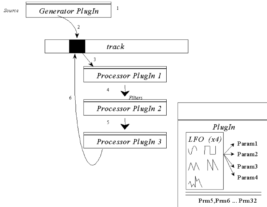
Fig. 5. Schematic showing the structure of the generators, processors and oscillators of one of the eight available audio channels, or tracks, on FMOL. Each track uses an independent audio buffer, a sound generator and three serial processors. The grey square represents the frame being computed at the time, and the numbers (1 to 6) show the order in which the internal steps are carried. This process is done at a rate of 25 frames per second for each track. Furthermore, each plug-in (both generators and processors) has four available oscillators that control the plug-in's four primary parameters (secondary parameters are used to dynamically control the frequency and the amplitude of the oscillators themselves).
